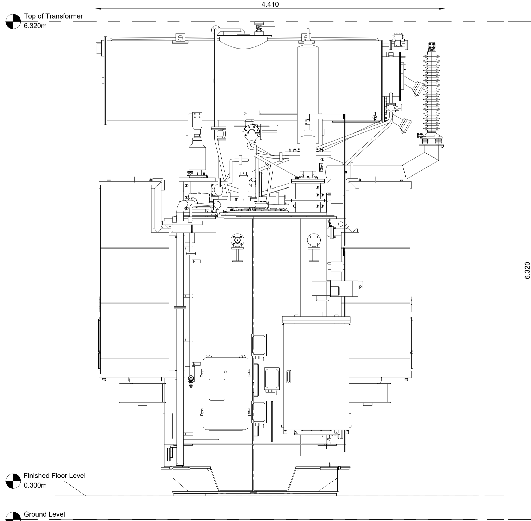
4 High Voltage Transformer West Elevation Scale 1:25 @ A1
